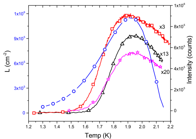
FIG. 10. Dependence of vortex density in superfluid helium, L , on temperature during observation of thermoluminescence from the ensemble of nitrogen nanoclusters (circles) 38 and temperature dependences of thermoluminescence intensity of \alpha -group nitrogen atoms for the different samples formed from [N_2]/[He] = 1/400 (squares), [N_2]/[Ar]/[He] = 1/1/200 (triangles), [N_2]/[Ne]/[He] = 1/1/100 (stars) gas mixtures.
