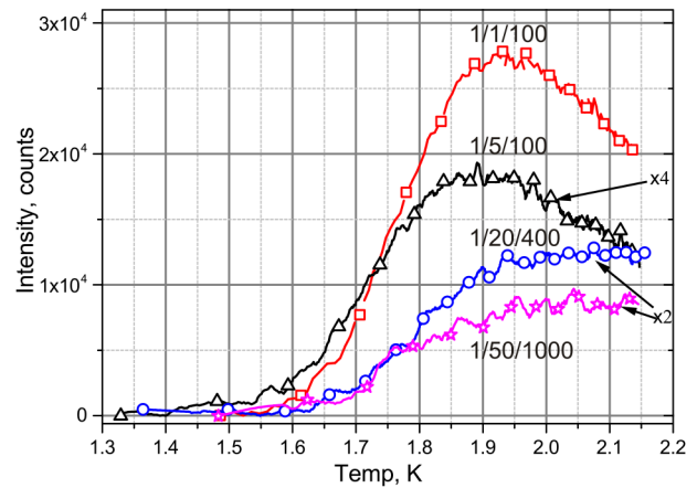
FIG. 7. Temperature dependences of thermoluminescence intensity of nitrogen atoms in nitrogen–neon nanoclusters formed from different nitrogen–neon–helium gas mixtures: 1/1/100 (red line with squares), 1/5/100 (black line with triangles) and 1/20/400 (blue line with circles), 1/50/1000 (magenta line with stars). Warming up to T \sim 2.15 K lasted 157, 212, 255, and 227 s, for curves from top to bottom, respectively.
