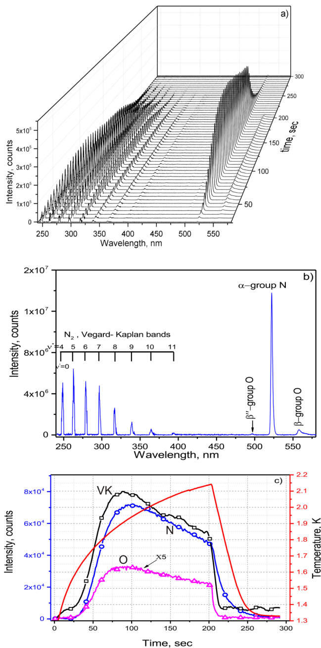
FIG. 2. Thermoluminescence of ensemble of nitrogen–argon nanoclusters immersed in superfluid helium. An ensemble of nanoclusters was prepared from gas mixture [^{14}N_2]/[Ar]/[He] = 1/1/200 . (a) Dynamics of thermoluminescence spectra of the ensemble of nanoclusters during warming up from 1.3 to 2.15 K. Each spectrum in the figure is a sum of 100 spectra taken with exposure time 50 ms. (b) Integrated thermoluminescence spectra obtained during entire warming process. (c) Time dependence of sample temperature (red line). Time dependences of thermoluminescence intensity for nitrogen molecules integrated over all observed VK bands (black line with squares), nitrogen atoms (blue line with circles) and oxygen atoms (magenta line with triangles).
