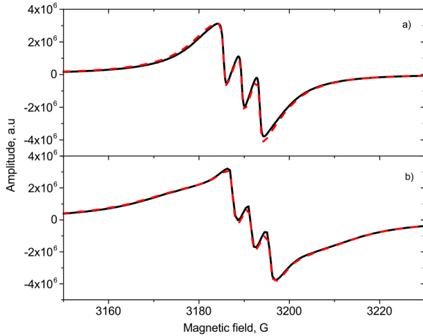
FIG. 8. Comparison of the ESR spectra for as-prepared ensembles of nanoclusters taken at T = 1.32 K (black solid line) and after completing cycle of warming to 2.16 K and cooling back to T = 1.32 K (red dashed line). Spectra were obtained for samples prepared from nitrogen–neon–helium mixture [N_2]/[Ne]/[He] = 1/1/100 (a), and nitrogen–argon–helium mixture [N_2]/[Ar]/[He] = 1/1/200 (b).
