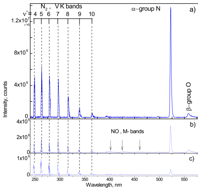
FIG. 4. Integrated thermoluminescence spectra obtained during warming of three ensembles of nitrogen–argon nanoclusters. Ensembles of nitrogen–argon nanoclusters were prepared from different [^{14}\text{N}_2]/[\text{Ar}]/[\text{He}] gas mixtures: (a) 1/1/200, (b) 1/5/600, (c) 1/20/2000.
