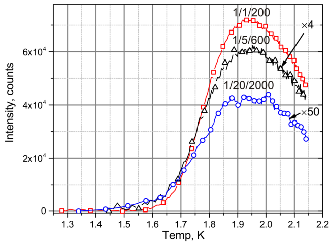
FIG. 3. Temperature dependences of thermoluminescence intensity of nitrogen atoms for ensembles of nanoclusters formed from different nitrogen–argon–helium gas mixtures: 1/1/200 (red line with squares), 1/5/600 (black line with triangles) and 1/20/2000 (blue line with circles). Warm up to T \sim 2.15 K lasted 202, 165, and 215 s, respectively.
