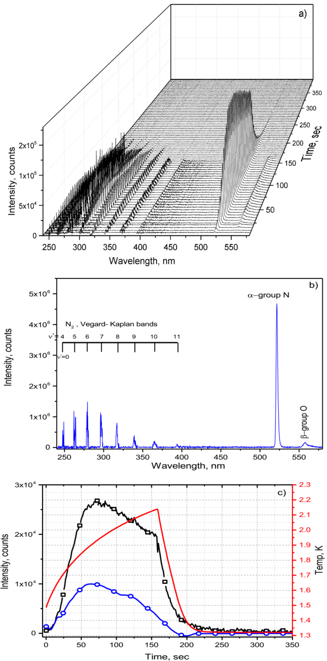
FIG. 5. Thermoluminescence of nitrogen–neon nanoclusters immersed in superfluid helium. Nanoclusters were prepared from gas mixture [^{14}\text{N}_2]/[\text{Ne}]/[\text{He}] = 1/1/100 . (a) Dynamics of thermoluminescence spectra of the nanoclusters during warming up from 1.3 to 2.15 K. Each spectrum in the figure is a sum of 100 spectra taken with exposure time 50 ms. (b) Integrated thermoluminescence spectra obtained during entire warming process. (c) Time dependences of sample temperature (red line). Time dependence of thermoluminescence intensity for VK bands of nitrogen molecules (blue line with circles), and \alpha -group of nitrogen atoms (black line with squares).
