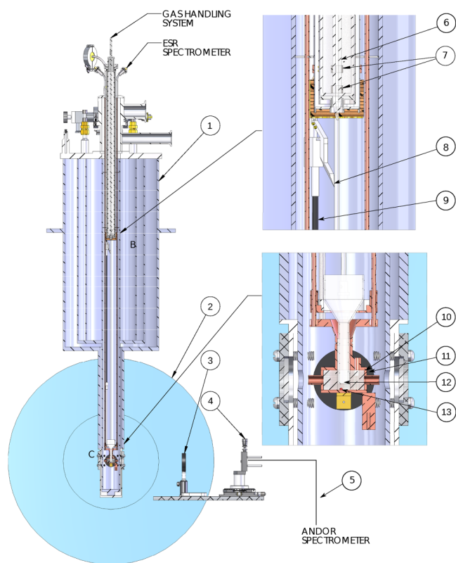
FIG. 1. Schematic of the setup for optical spectroscopy and electron spin resonance studies of the ensembles of nanoclusters immersed in superfluid helium: 1—cryostat, 2—magnet, 3—lens for collecting light emitted from the sample, 4—optical stage, 5—fiber optics, 6—quartz tube, 7—discharge electrodes, 8—teflon blade, 9—liquid helium level meter, 10—microwave cavity with optical access, 11—modulation coil, 12—sample collection beaker, 13—ruby crystal.
