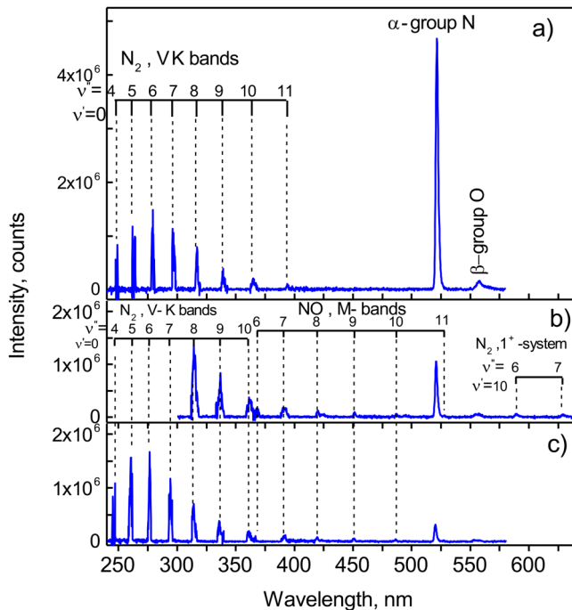
FIG. 6. Integrated luminescence spectra obtained during warming of three ensembles of nitrogen–neon–nanoclusters. Nitrogen–neon nanoclusters were prepared from [^{14}\text{N}_2]/[\text{Ne}]/[\text{He}] gas mixtures: (a) 1/1/100, (b) 1/20/400, (c) 1/50/1000.
