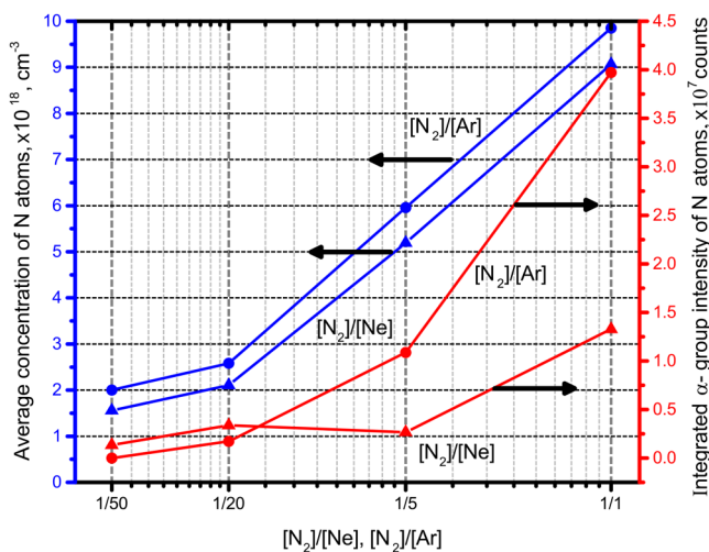
FIG. 9. Dependence of the average concentration of N atoms stabilized in nitrogen–neon and nitrogen–argon nanoclusters on the N_2/Ne (blue line with triangles) and N_2/Ar (blue line with circles) ratios in gas mixtures. Dependence of the integrated \alpha -group intensity of nitrogen atoms during the warming in ensembles of nitrogen–neon and nitrogen–argon nanoclusters on the N_2/Ne (red line with triangles) and N_2/Ar (red line with circles) ratios in gas mixtures. Arrows correspond to right and left hand vertical scales, respectively.
