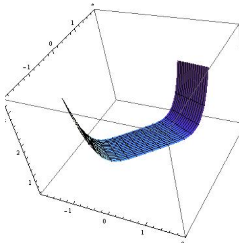
Figure 1. Spherical Orthotomic Timelike Ruled Surface
