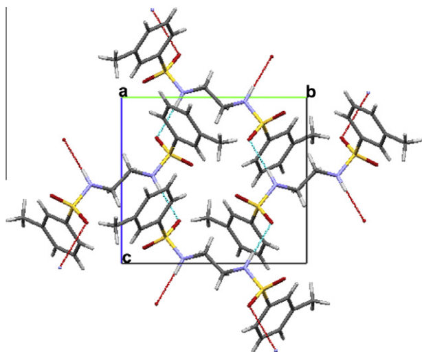
Fig. 2. Unit-cell packing diagram of mtsen.
