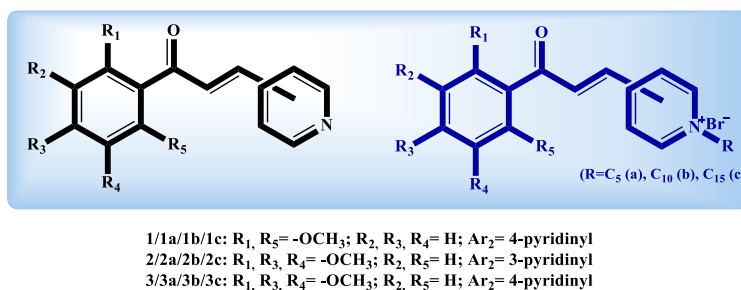
Figure 1. Structures of newly synthesized azachalcones and N -alkyl derivatives
