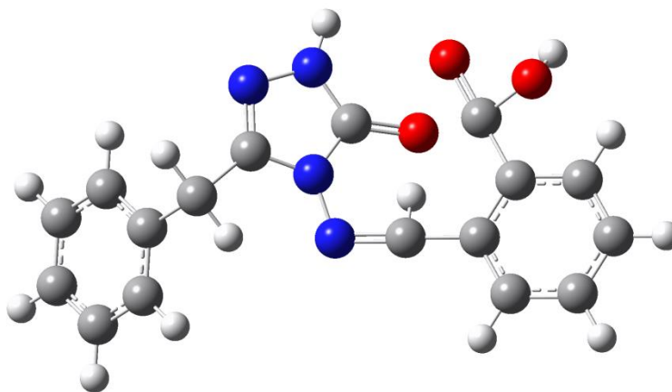
The Gaussview structure of the molecule
