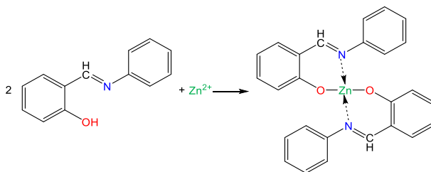
Fig. 1. Synthesis of \text{Zn}^{2+} -HL complex
