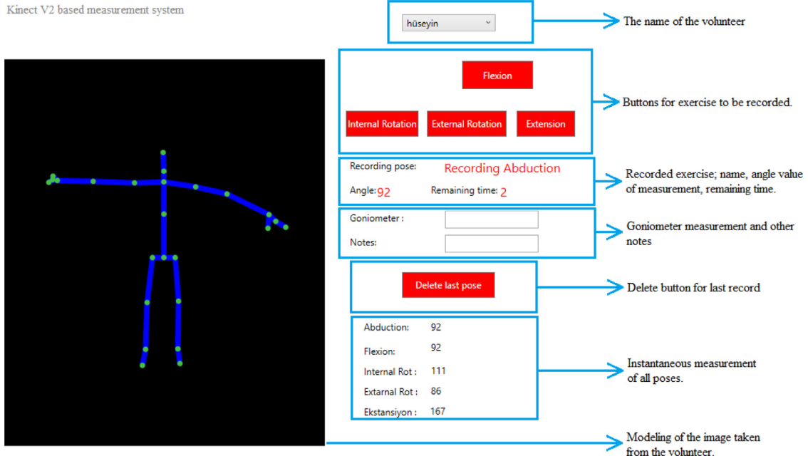
Figure 4. Developed GUI for reliability and validity tests.
