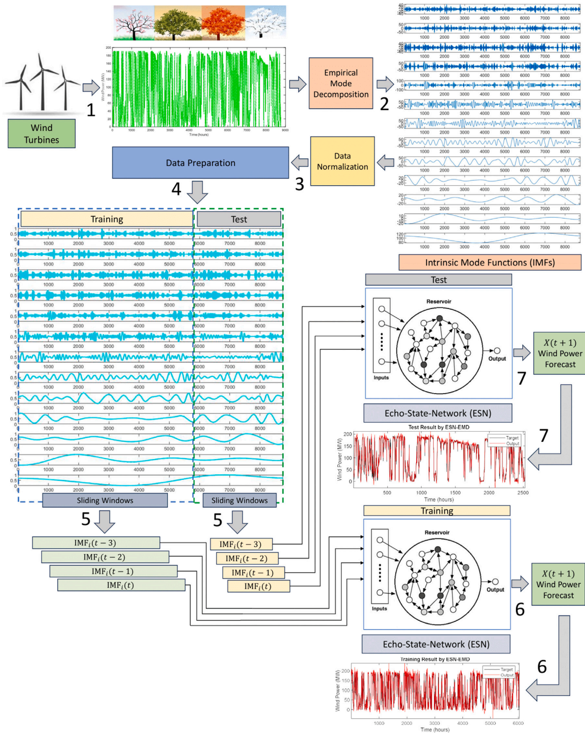
Fig. 2. Framework of hybrid EMD-ESN model.
