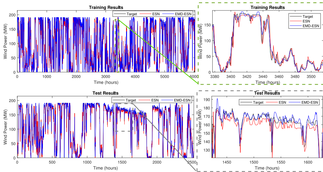
Fig. 4. The training and test results of the proposed EMD-ESN hybrid model for West of Duddon Sands dataset.
