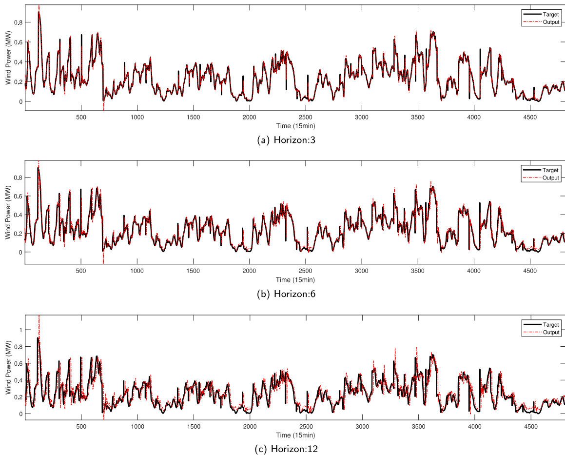
Fig. 7. EMD-ESN model's test results for 3-6-12-step wind power forecasting.
