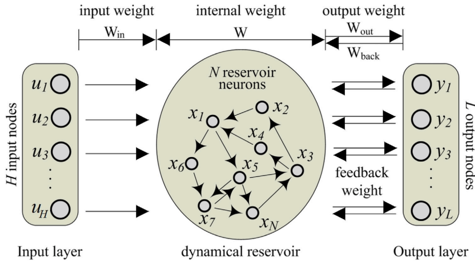
Fig. 1. ESN model architecture [40].
