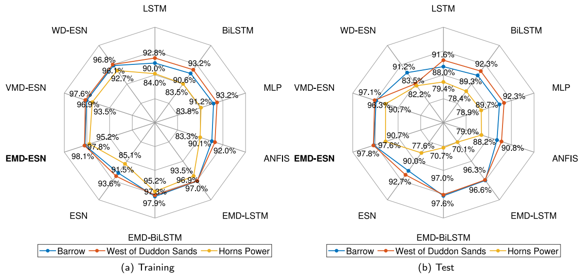
Fig. 6. R^2 results of EMD-ESN and other models for offshore datasets.
