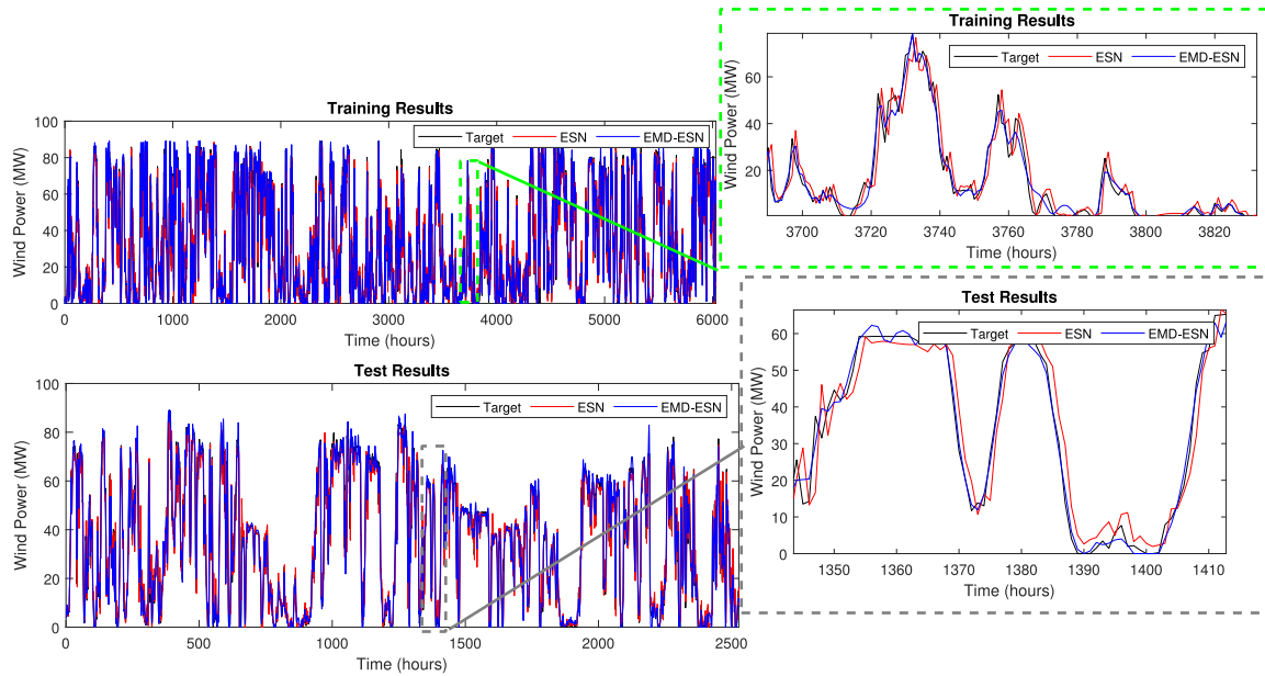
Fig. 3. The training and test results of the proposed EMD-ESN hybrid model for Barrow dataset.
