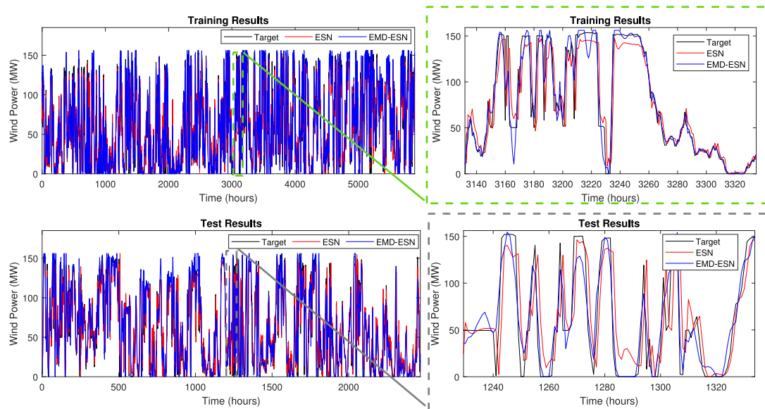
Fig. 5. The training and test results of the proposed EMD-ESN hybrid model for Horns Power dataset.
