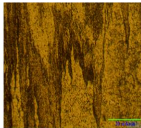
Fig 2.14 FSW test sample of AA5754 b and the region c micrograph (X50)
