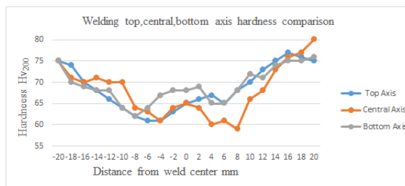
Fig 2.17 1600 rev/min rotation and 125 mm/min feed rate to the top of the line joining the welding made from the cross-sectional area, a graphical representation of the upper, middle and lower axis.
