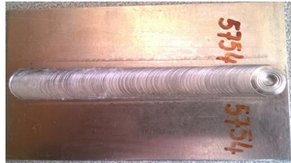
Fig 2.6 With friction stir welding method macrograph of accurate combined AA 5754 aluminum alloy sheet
