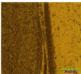
Fig 2.13 FSW test sample of AA5754 a, b and c of micrograph (X50)
