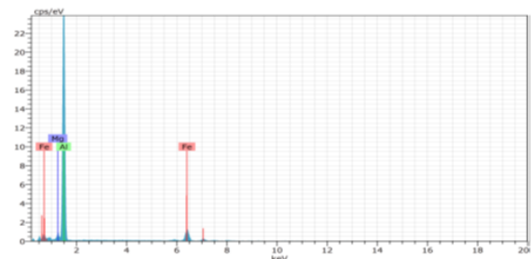
Fig.2.23 Scanning electron microscope (SEM) EDS spectrum of the HAZ, TMAZ and SZ.
