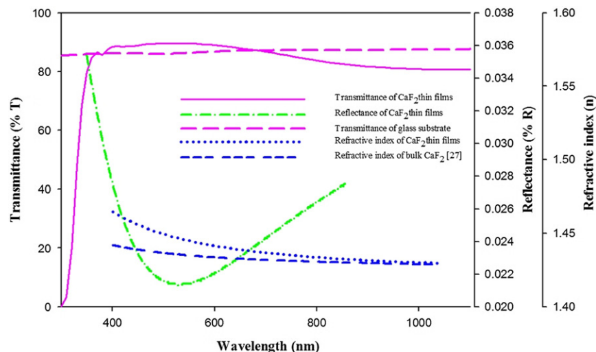
Fig. 4. Transmission and reflection spectra along with the wavelength dependency of the refractive index for a typical \text{CaF}_2 thin film sample.
