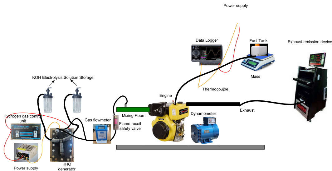
Fig. 3 – Schematic view of the experimental setup.
