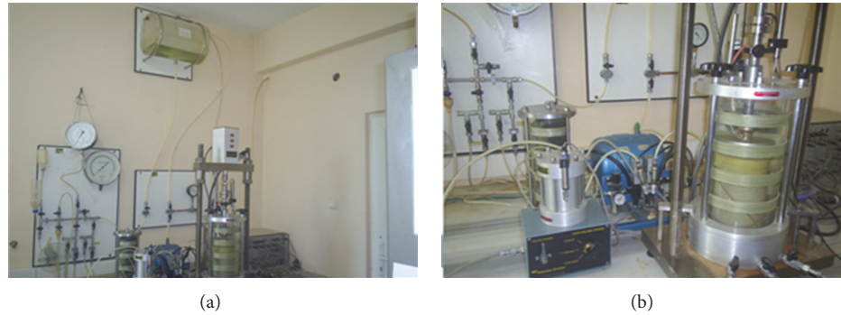
FIGURE 2: The cyclic triaxial test system.
