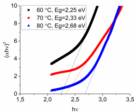
Figure 4. Tauc plots and estimated band gaps of the CdO samples
