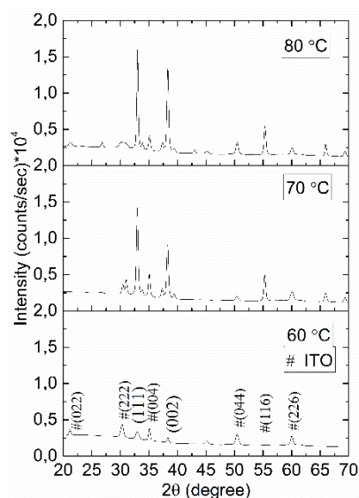
Figure 1. The XRD patterns of the CdO samples
