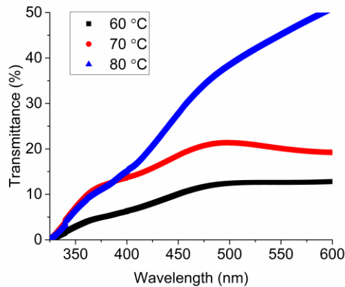
Figure 3 Transmittance values of the CdO films
