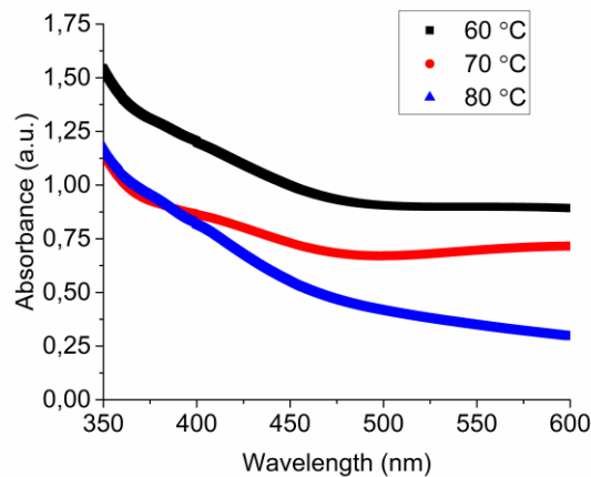
Figure 2. Absorbance values of the CdO films
