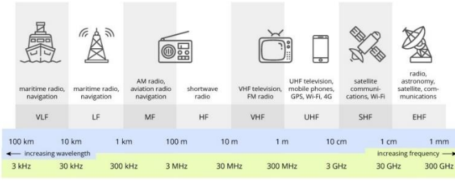
Figure 3 Wireless Radio Frequencies.
