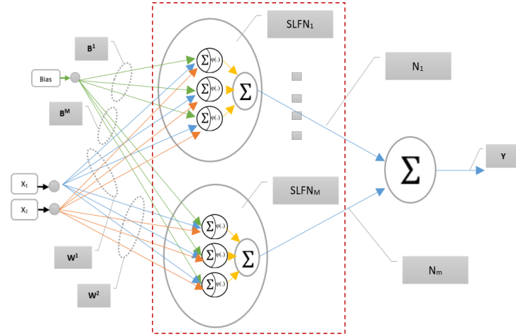
Figure 2 The Meta-ELM Architecture with 2 group ( M=2 ) and 3 neuron ( N=3 ).
