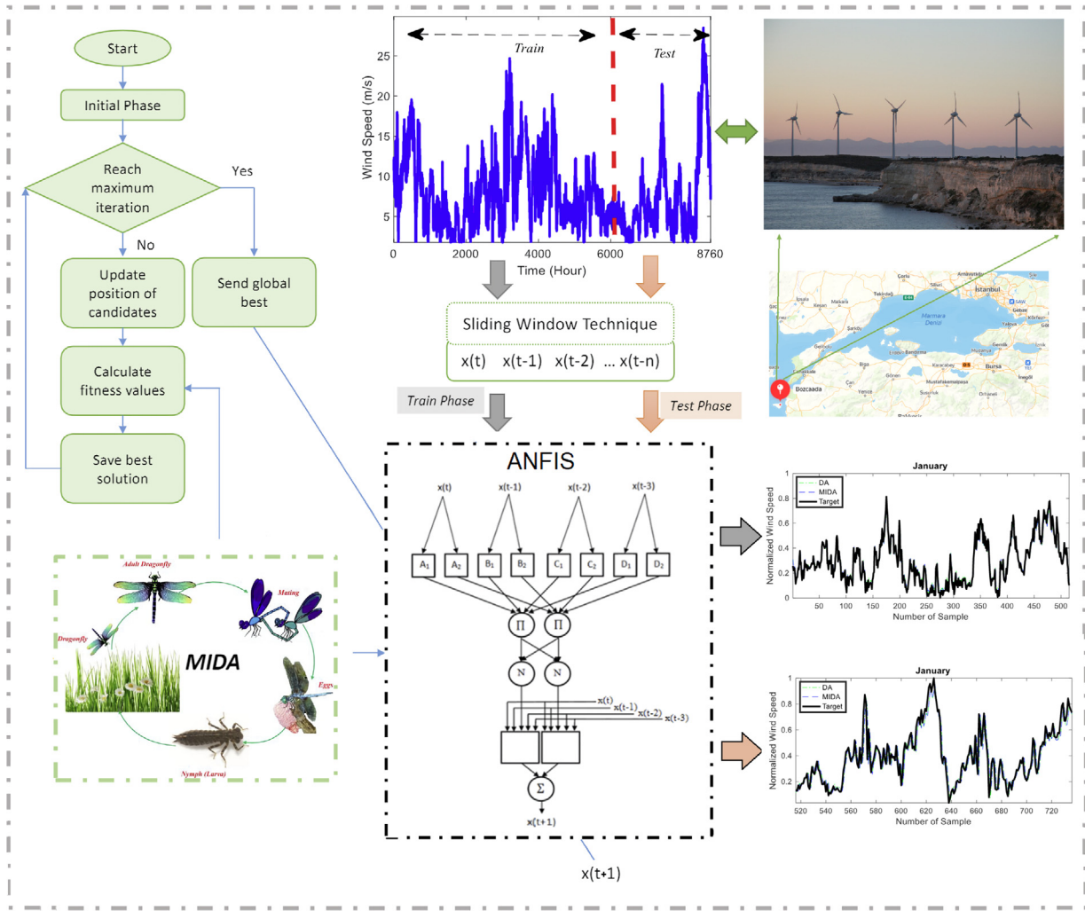
Fig. 16. The structure of the ANFIS and MIDA hybrid forecasting model.
