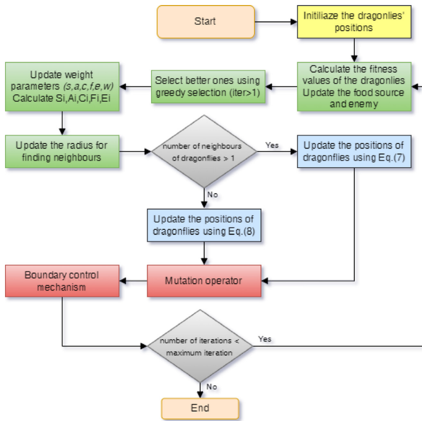
Fig. 2. Flowchart of MIDA.
