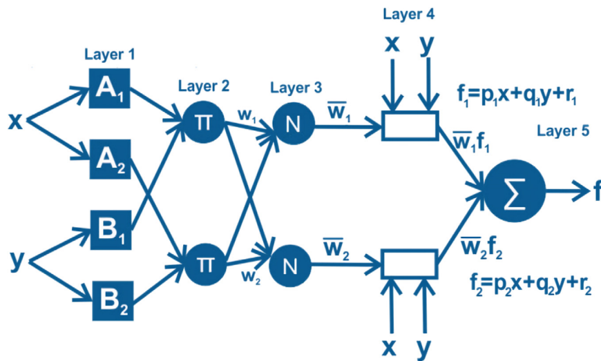
Fig. 3. General ANFIS model architecture [72].
