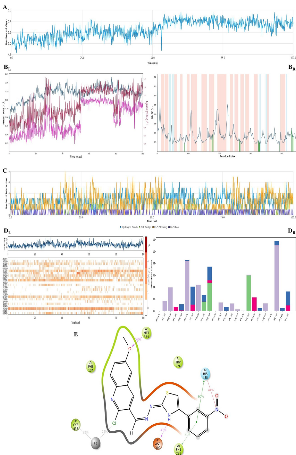
Figure 8. Plots of the MDS results for compound 4i –aromatase enzyme complex. The stability properties ( R_g , RMSD, and RMSF plots, respectively) are in (A) and (B) sections. The interaction properties ((C) number of interactions–interaction types–time plot; (D R ) interaction fraction–residue diagram; (D L ) total connections–residues–time plot; and (E) 2D interaction pose with connection strength (cutoff = 0.2) at the active region) are in (C)–(E) sections.
