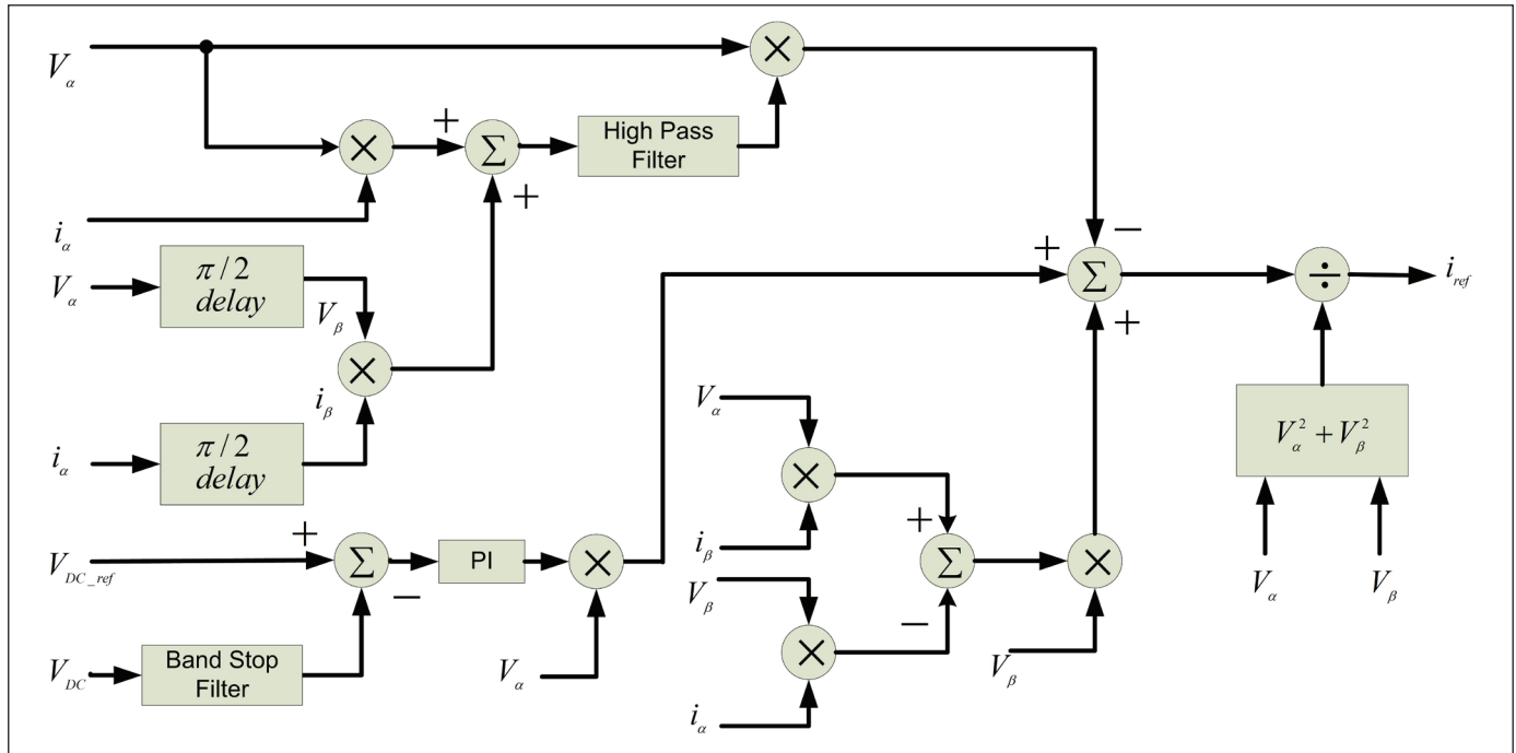
Figure 1. Improved controller schema for bridgeless PFC rectifier.
