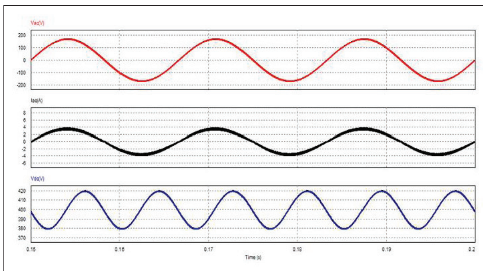
Figure 6. The input voltage and current, output voltage waveforms for 300W BBPFC rectifier with average current control (PF 0.9894, THD %5.51).
