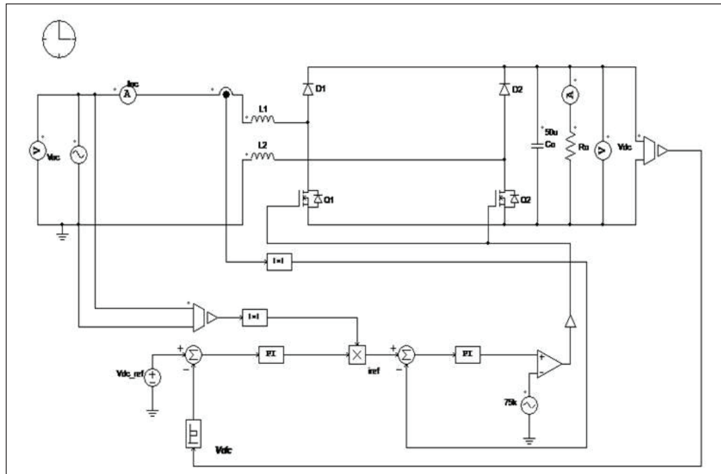
Figure 4. PSIM simulation circuit for 300W BBPFC rectifier with average current control.
