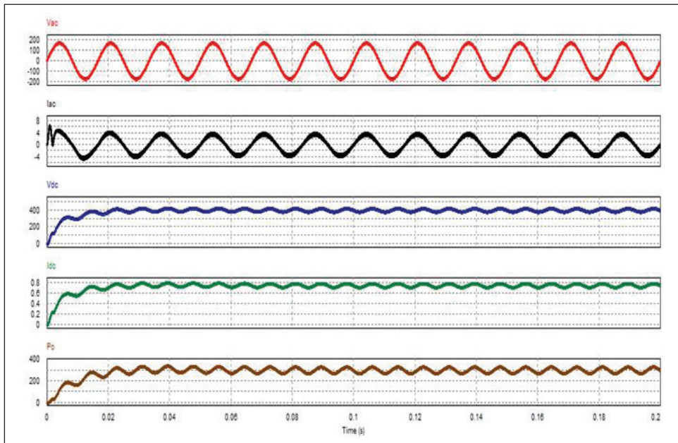
Figure 5. The transient input voltage, input current, output voltage, output current and output power for 300W BBPFC rectifier with average current control.
