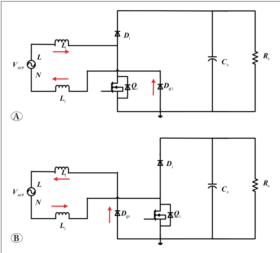
Figure 3. Bridgeless boost BPFC rectifier operation mode with (A) positive and (B) negative line cycle.
