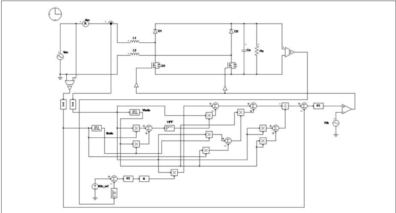
Figure 7. PSIM simulation circuit for 300W BBPFC rectifier with pq controller.
