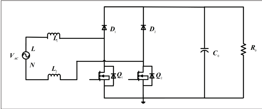
Figure 2. Bridgeless boost PFC rectifier circuit.
