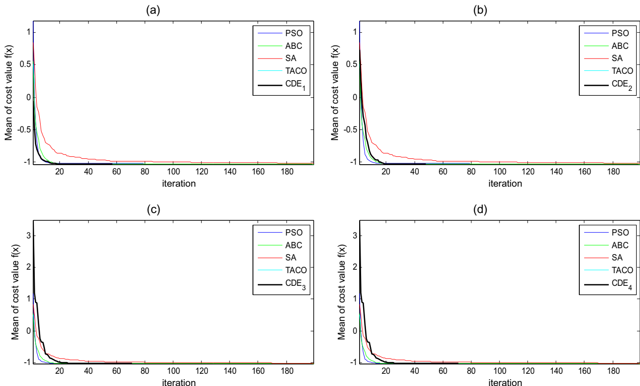
Fig. 3. Average best fitness curves of CDE Algorithms and PSO, ABC, SA and TACO algorithms for test function FN9. All experimental results are means of 50 independent runs. (a) Lorenz based DE Algorithm. (b) Rossler based DE Algorithm. (c) Chua based DE Algorithm. (d) Mackey-Glass based DE Algorithm.
