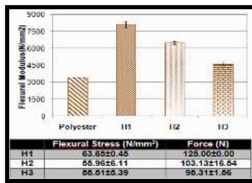
Figure 2: Some properties of hops composite material's ability to resist deformation
