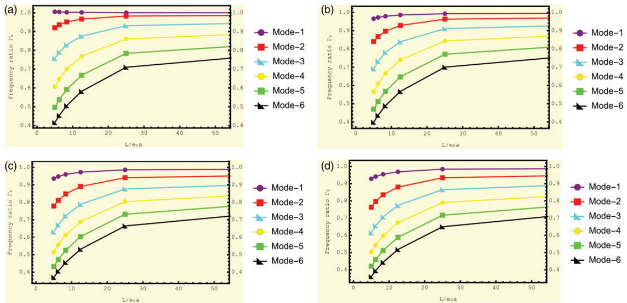
Figure 15. The effect of elastic spring coefficients ( \Phi_0, \Phi_L ) on the torsional vibration frequencies.
