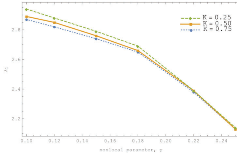
Figure 14. First torsional vibration frequency as a function of nonlocal parameter for \Delta_I = 0.45 .
