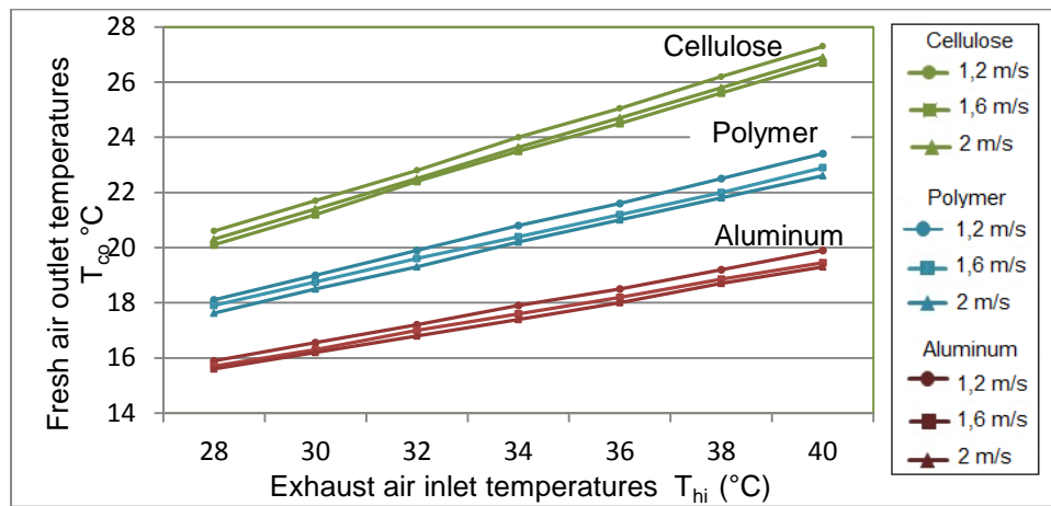
Fig. 5 Comparison of the fresh air outlet temperatures of the aluminum, polymer and cellulose heat exchangers at different air rates when fresh air inlet temperature is 10 °C
