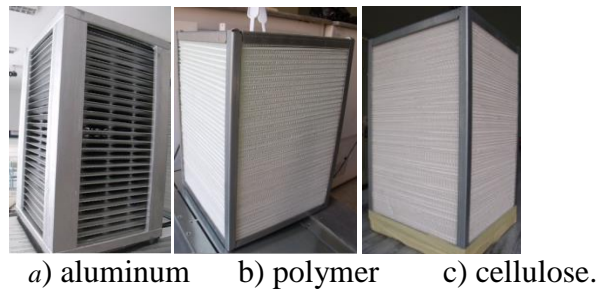
Fig. 1 The heat exchangers used in the apparatus
