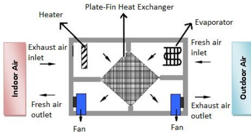
Fig. 2 Schematic representation of the testing apparatus
