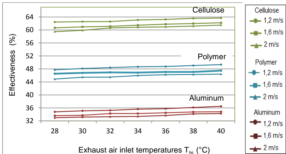
Fig. 6 Comparison of effectiveness of the aluminum, polymer and cellulose heat exchangers where the fresh air inlet temperature is 0 °C at different air rates
