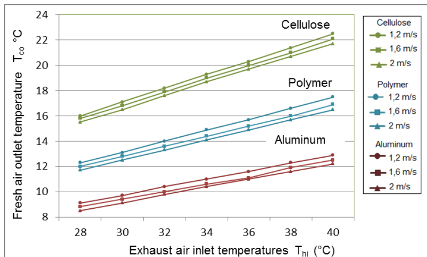
Fig. 4 Comparison of the fresh air outlet temperatures of the aluminum, polymer and cellulose heat exchangers at different air rates when the fresh air inlet temperature is 0 °C
