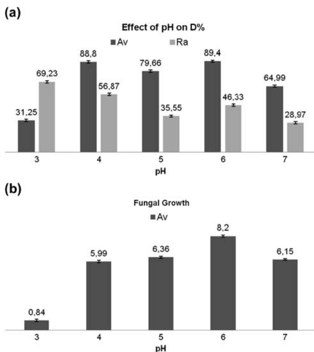
Fig. 1. (a) The effect of pH on decolorization (D%) by growing cultures and (b) the effect of pH on fungal growth of A. versicolor (Av: A. versicolor ; Ra: R. arrhizus ; C_{ORB} : 100 mg/L; incubation period: six days; T : 25 \pm 1^\circ\text{C} ).
