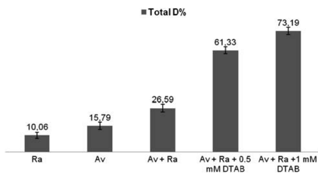
Fig. 4. Total decolorization (D%) activity (Av: A. versicolor ; Ra: R. arrhizus ; Av + Ra: mixed A. versicolor and R. arrhizus ; DTAB: dodecyl trimethyl ammonium bromide; C_{\text{ORB}} : 800 mg/L; incubation period: three days; T : 25 \pm 1^{\circ}\text{C} ).
