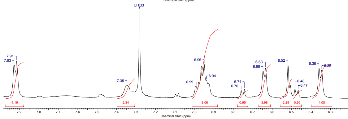
Bileşik C3 ^1\text{H} -NMR Spektrumu ( \text{CDCl}_3 , 500 MHz)
