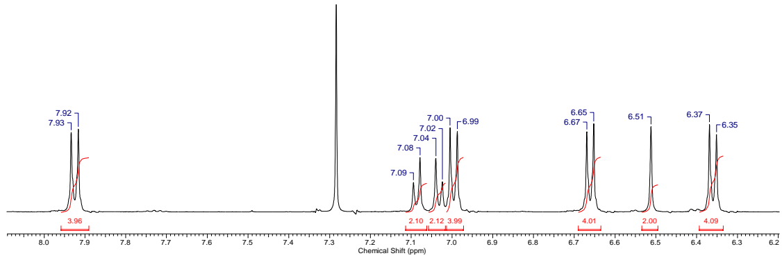
Bileşik C2 ^1\text{H} -NMR Spektrumu ( \text{CDCl}_3 , 500 MHz)
