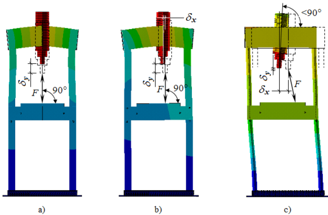
Figure 5. Vertical and horizontal displacements of the presses with N type head and S2 column under a) axial force, b) eccentric force, and N type head and S3 column under c) oblique force in the xy-plane
