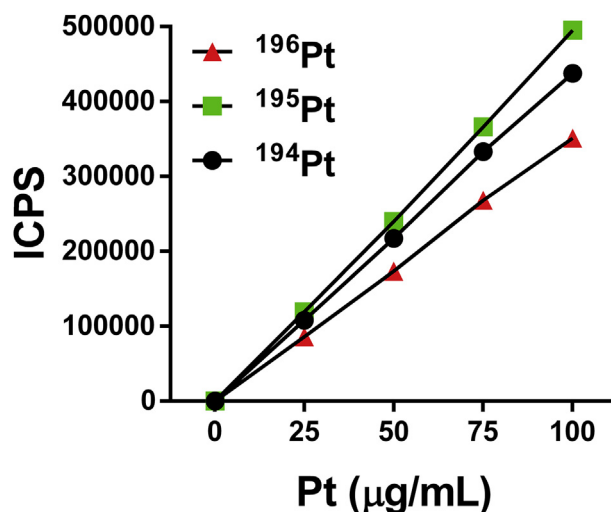
Fig. 1. Calibration graph and the best line equation for ^{194}\text{Pt} , ^{195}\text{Pt} and ^{196}\text{Pt} isotopes by ICP-MS.
