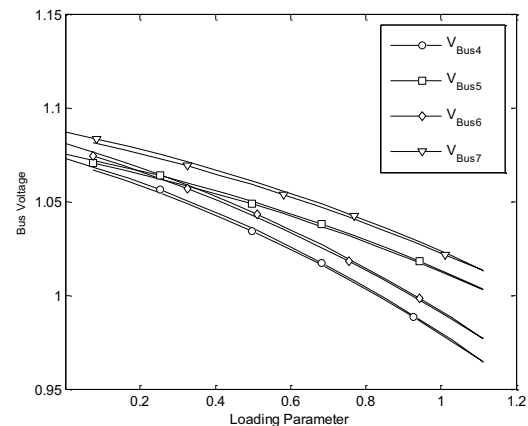
Fig. 10 With SSSC 4, 5, 6, 7 Bus Loading Parameter
