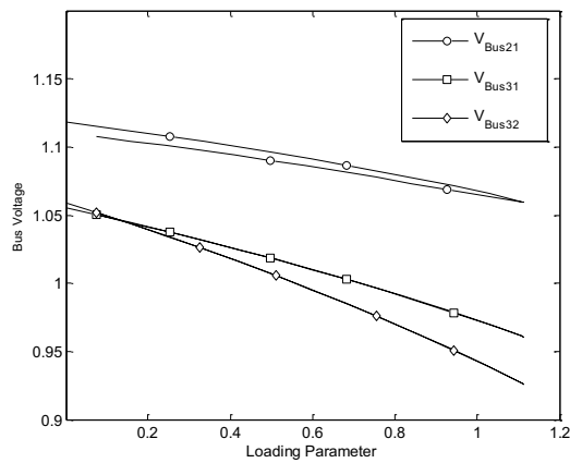
Fig. 11 With SSSC 21, 31, 32 Bus Loading Parameter
