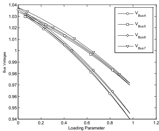
Fig. 6 Without FACTS 4, 5, 6, 7 Bus Loading Parameter
