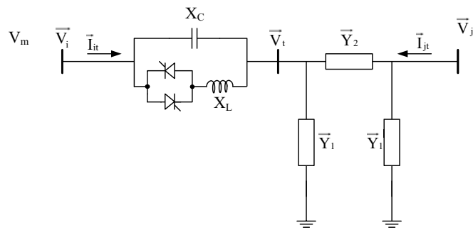
Fig. 1 TSSC Models
