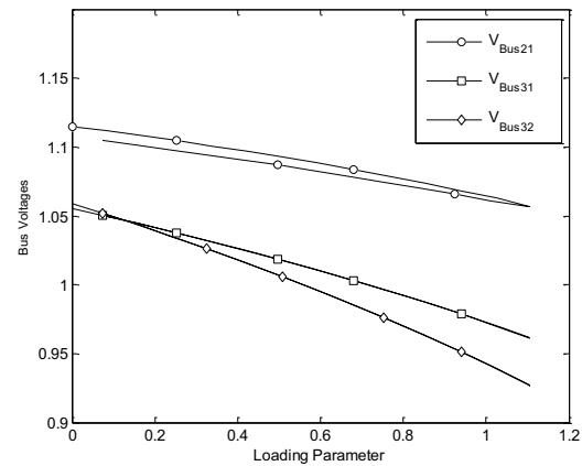
Fig. 9 With TCSC 21, 31, 32 Bus Loading Parameter
