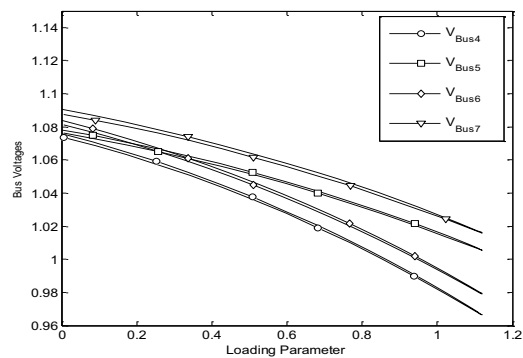
Fig. 12 With UPFC 4, 5, 6, 7 Bus Loading Parameter
