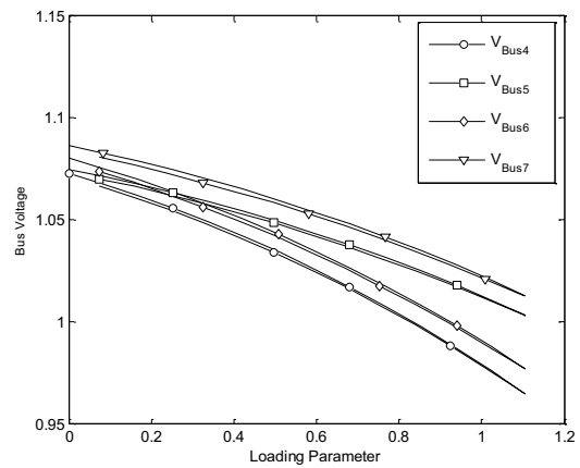
Fig. 8 With TCSC 4, 5, 6, 7 Bus Loading Parameter
