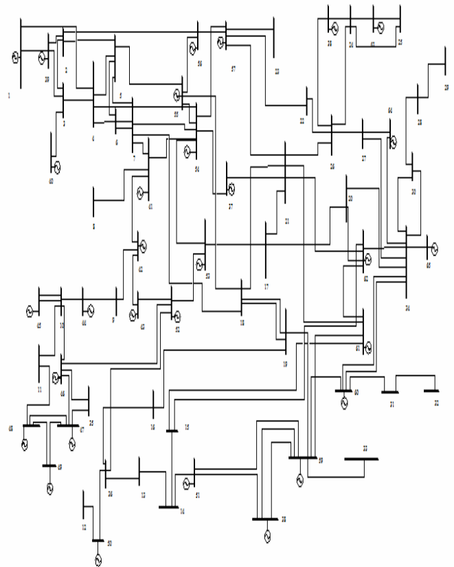
Fig. 5 65 Bus System
