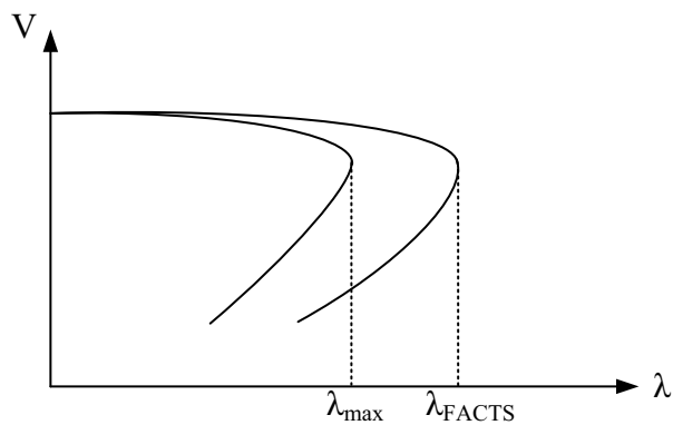
Fig. 4 Relation Voltage-Maximum Loading Parameter with FACTS
