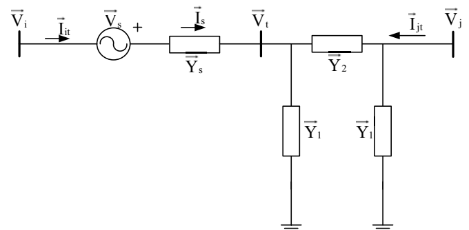
Fig. 3 UPFC Models
