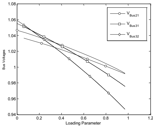
Fig. 7 Without FACTS 21, 31, 32 Bus Loading Parameter
