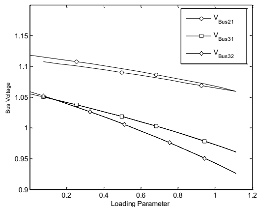
Fig. 13 With UPFC 21, 31, 32 Bus Loading Parameter
