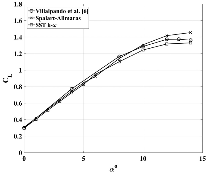
Fig. 6. Comparison between the computational C_L data of the current study and the numerical data of Villalpando et al. [6] for Re = 5 \times 10^5 .
