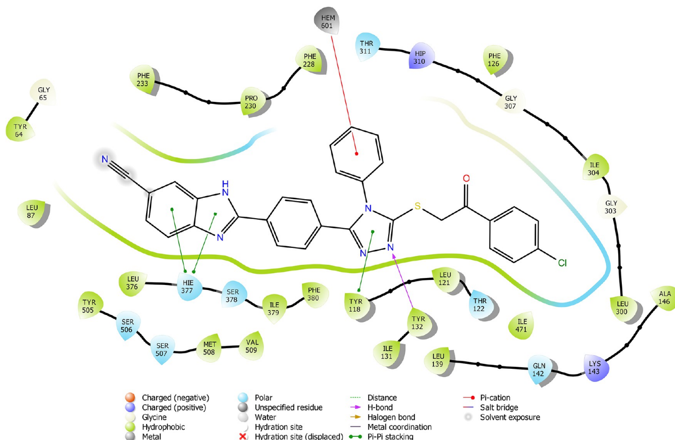
Figure 7. 2D schematic protein–ligand interactions of compound 6i in the active site of lanosterol 14 \alpha -demethylase (PDB ID: 5TZ1).
