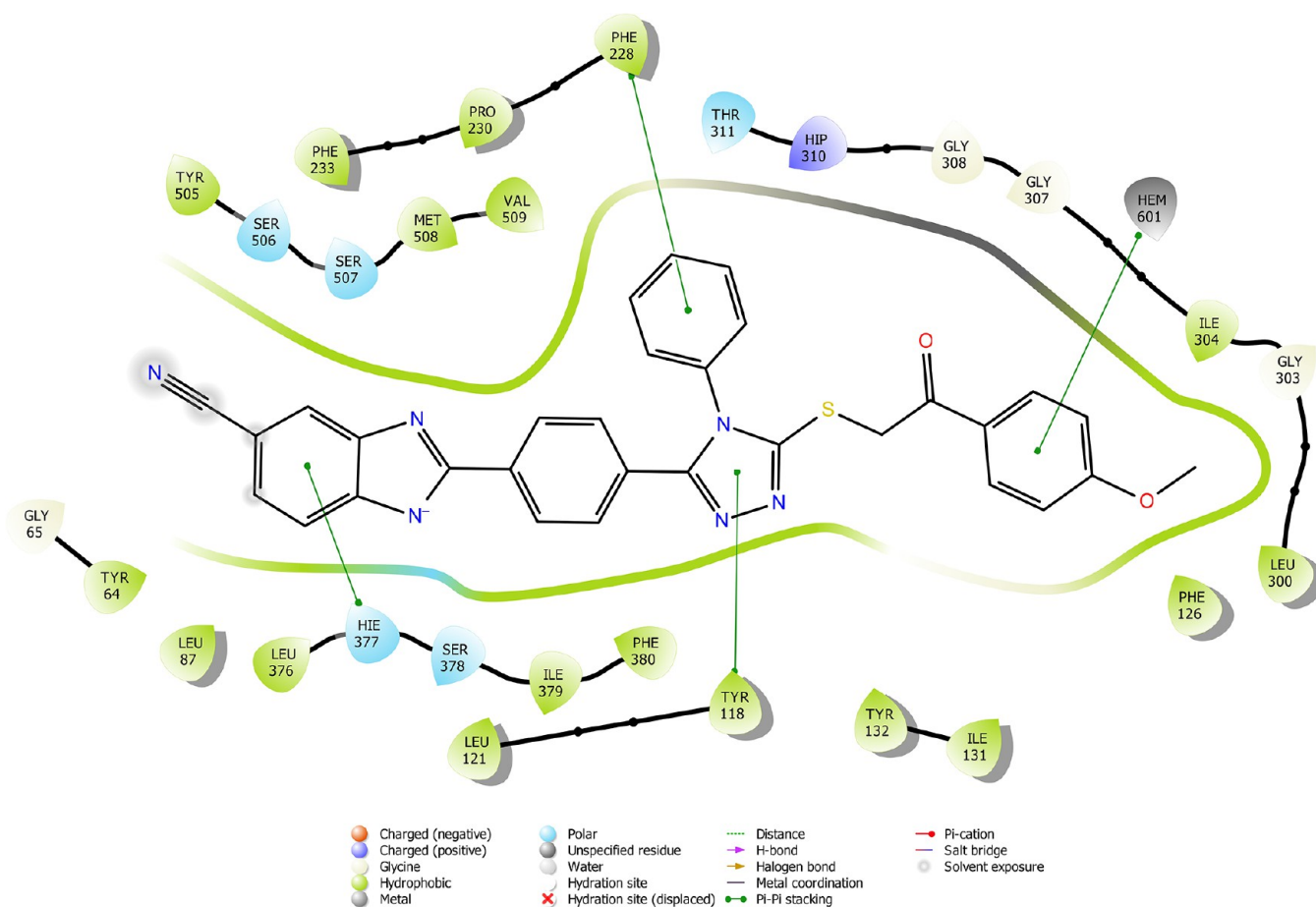
Figure 6. 2D schematic protein–ligand interactions of compound 6b in the active site of lanosterol 14 \alpha -demethylase (PDB ID: 5TZ1).
