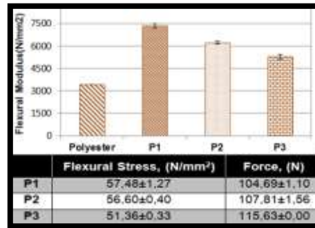
Figure 2: Some properties of pine cone composite material's ability to resist deformation
