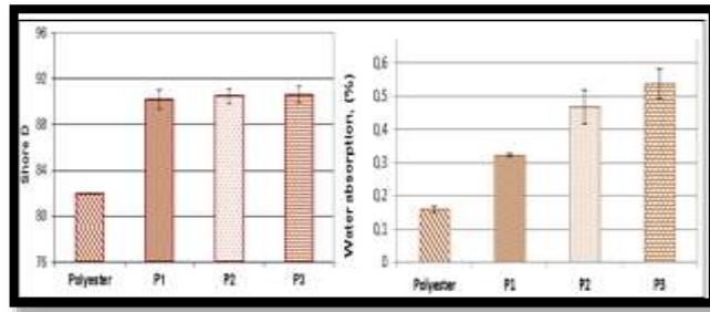
Figure 3: Physical testing results of pine cone/marble waste polyester matrix
