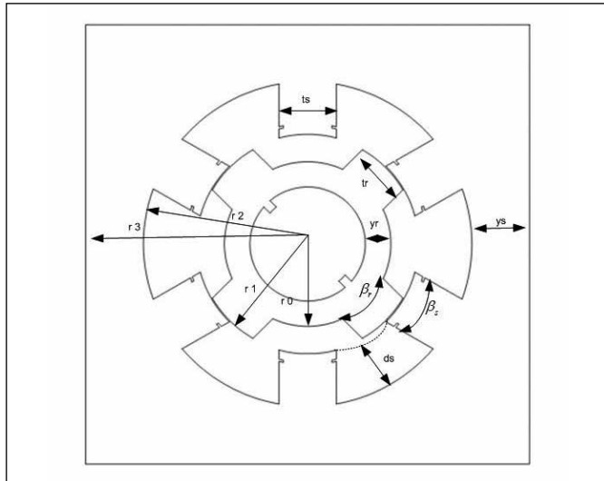
Figure 3. Geometric structure of the proposed MCSRSM.
