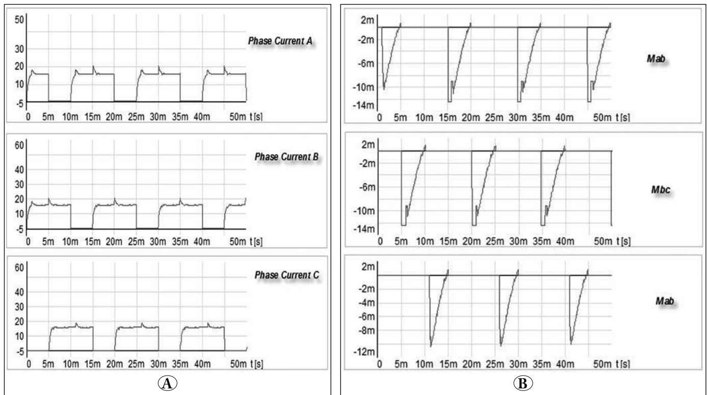
Figure 9. A) Phase currents. B) Mutual Inductances
