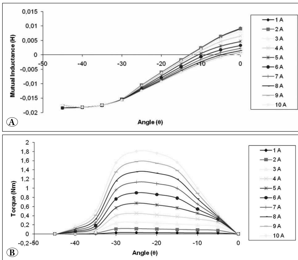
Figure 4. Mutual inductance and torque curves of the proposed MCSRSM. A) Mutual inductance variation of the proposed MCSRSM at different currents. B) Torque variation of the proposed MCSRSM at different currents.
