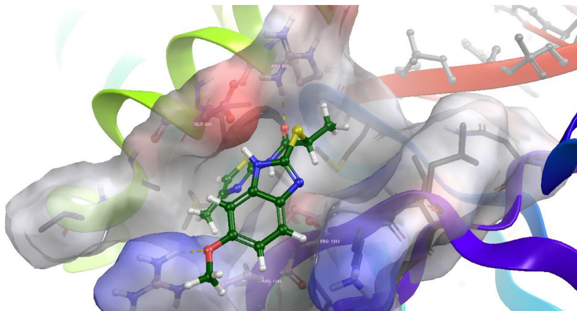
Fig. 4. Compound 3f in active site as 3D pose. Red line represents the DNA chain. (PDBID: 5NPK).
