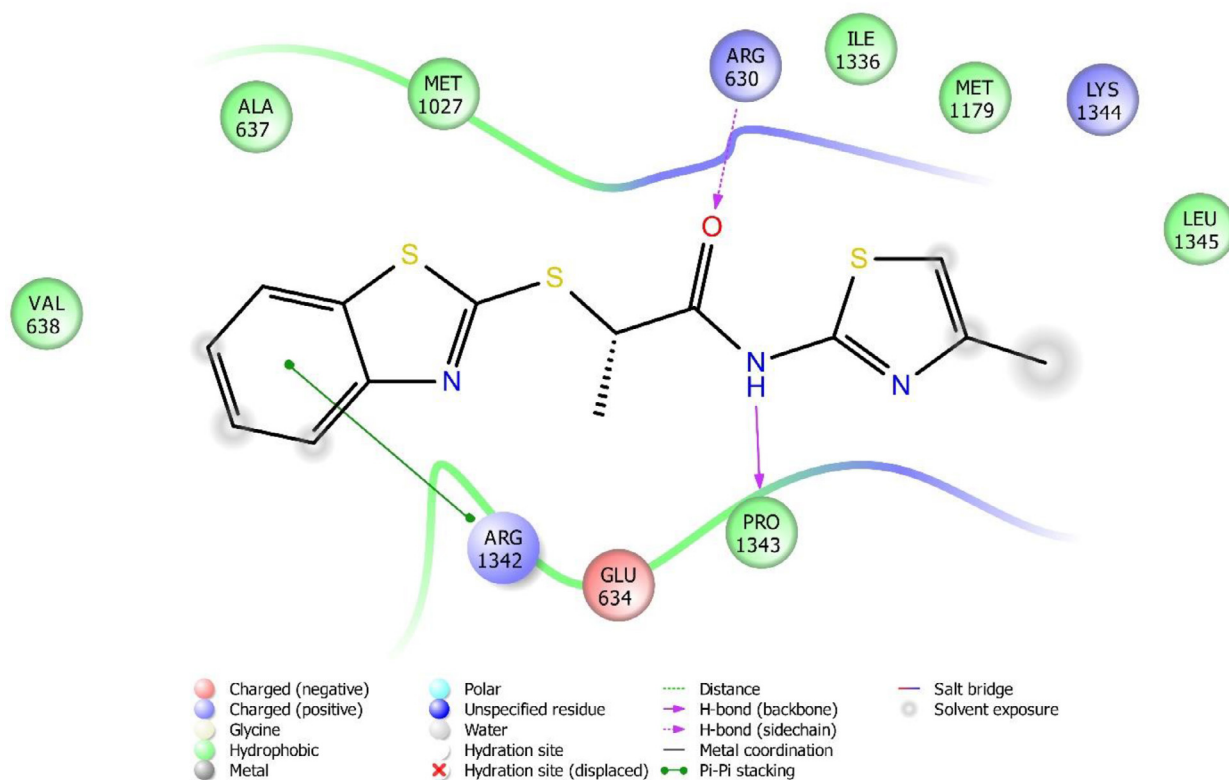
Fig. 5. 2D interaction diagram of compound 3i in active site. (PDBID: 5NPK).
