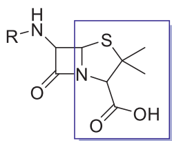
Fig. 1. The main structure of penicillins.
