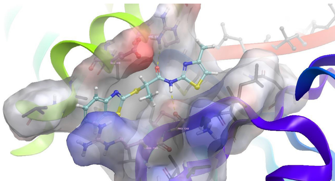
Fig. 6. Compound 3i in active site as 3D pose. Red line represents the DNA chain.
