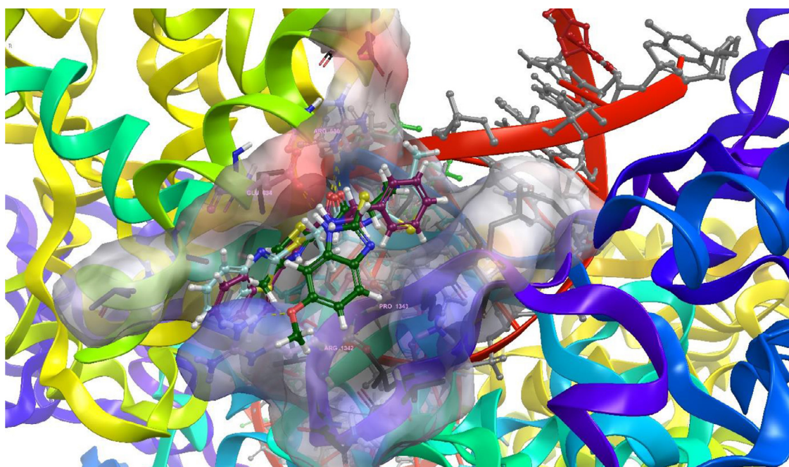
Fig. 2. Compounds 3f (green carbons) and 3i (turquoise carbons), and reference compound (maroon carbons) in DNA gyrase allosteric pocket (PDBID: 5NPK). The active site residues were drawn in stick form (black carbons). If there is an interaction between ligand and residue, these residues were represented in a ball-stick form (plum carbons). Red line represents the DNA chain.
