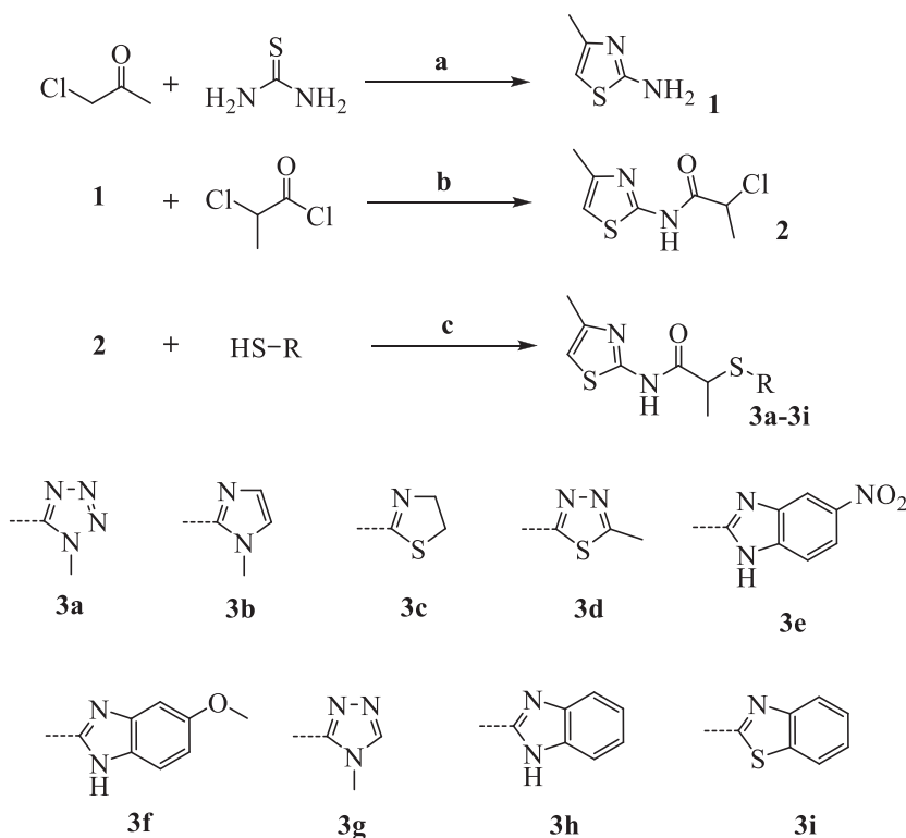
Scheme 1. The synthesis diagram of the compounds 3a–3i . Reagents and conditions: (a) EtOH, r.t., 24 h; (b) TEA, THF, ClCOCH 2 Cl, 0–5 °C, then r.t 3 h; (c) Acetone, K 2 CO 3 , r.t.
