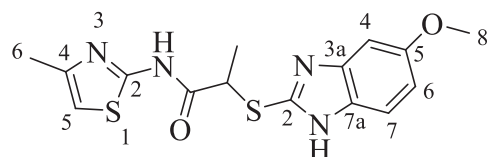
Scheme 2. As numbered the molecular structure of compound 3f .
