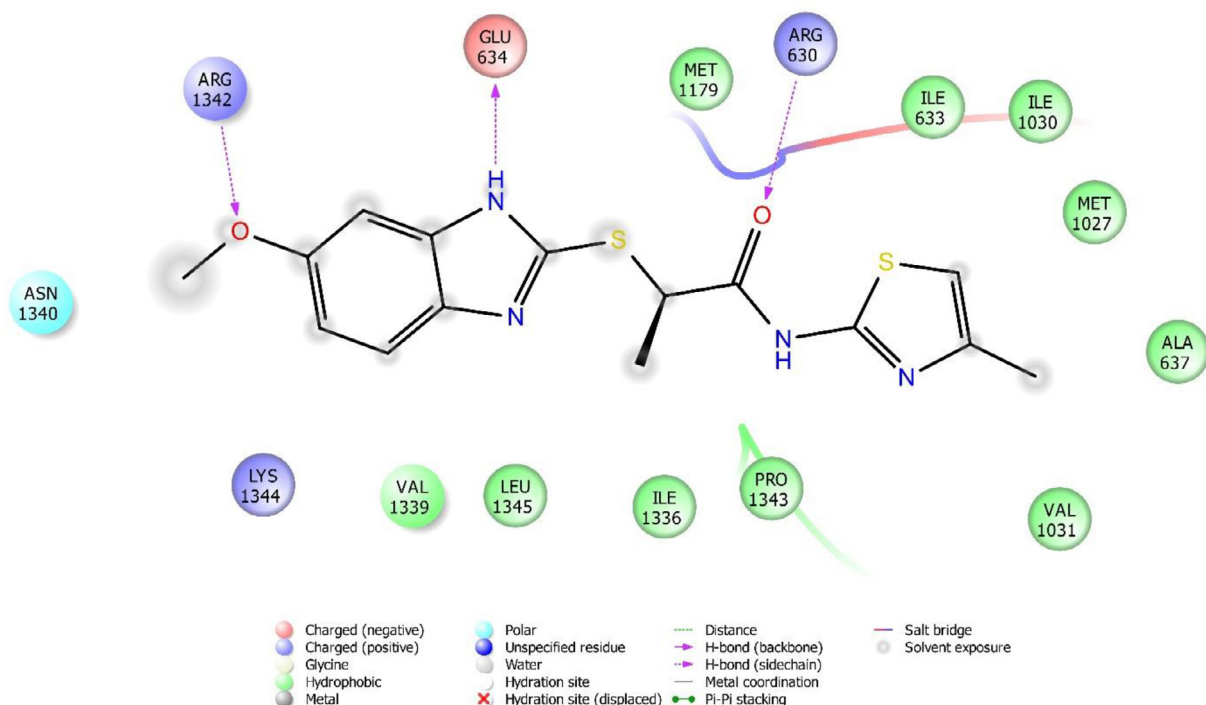
Fig. 3. 2D interaction diagram of 3f in active site. (PDBID: 5NPK).
