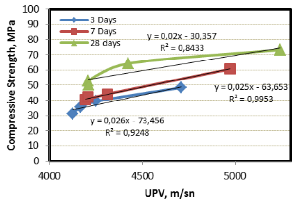
Figure 6. Relationship between compressive strength and UPV
