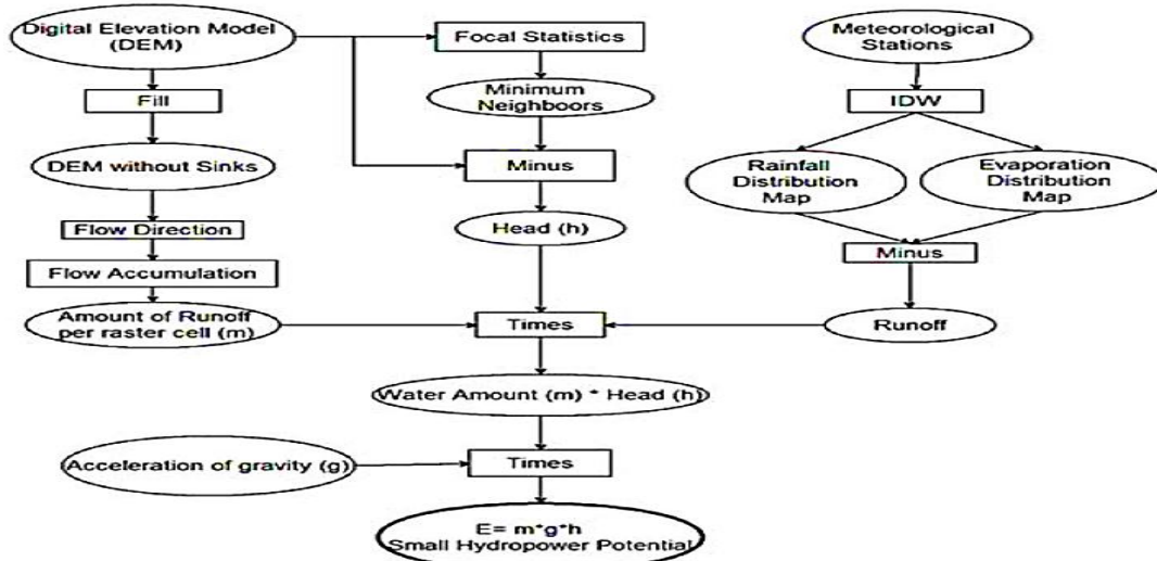
Figure-1. Flowchart of dam site selection method by using GIS (Bayazit et al., 2017).
