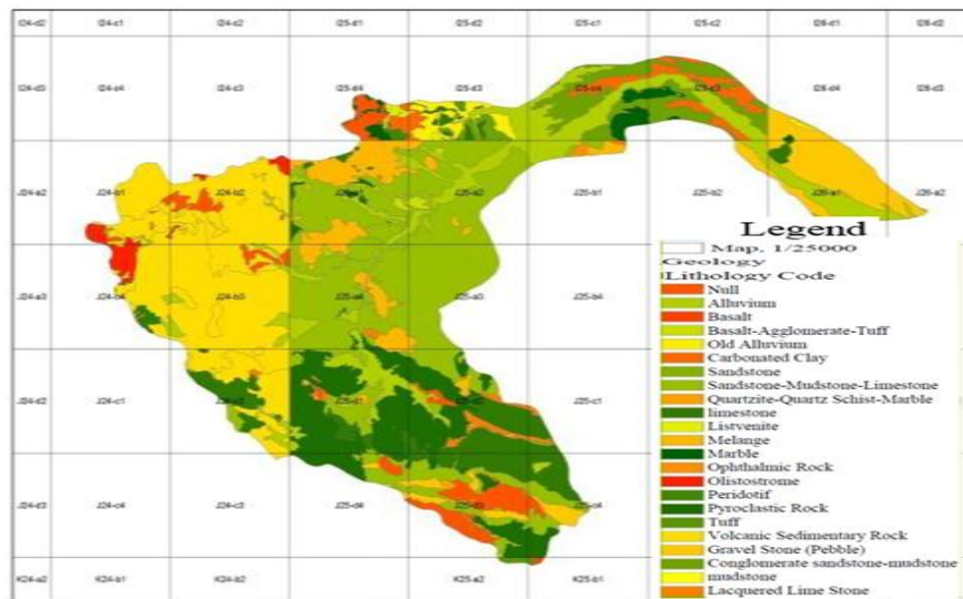
Figure-6. Geological map of the basin.
