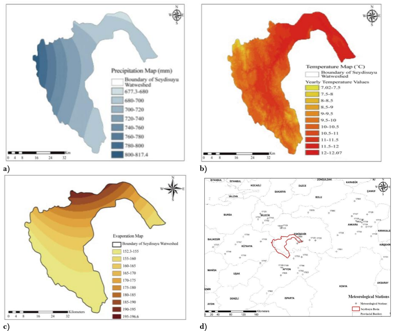
Figure-7. Distribution maps of meteorological features of Seydisuyu basin a) Precipitation (mm), b) Temperature (°C) c) Evaporation (mm) d) Meteorological stations.
