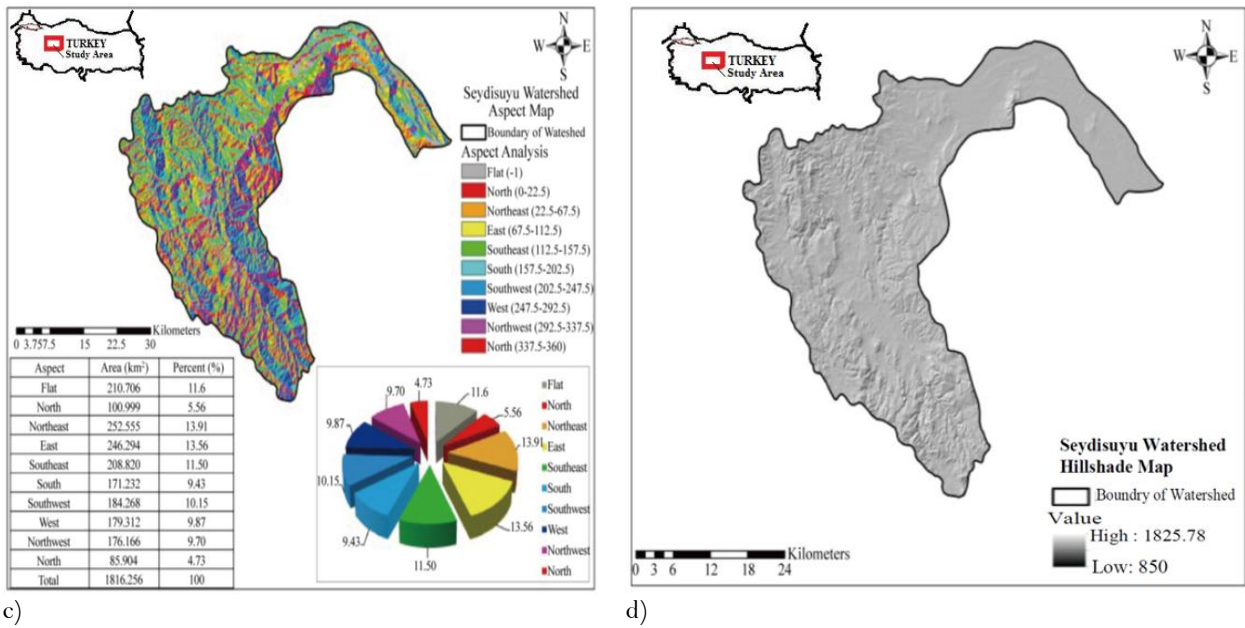
Figure-5. Thematic maps of Seydisuyu Basin a) Elevation-Topographic map; b) Slope map; c) Aspect map; d) Hill shade map.
