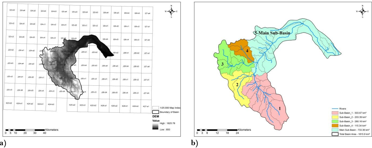
Figure-4. Seydisuyu Basin a) Digital Elevation Model (DEM) b) Sub-basins.
