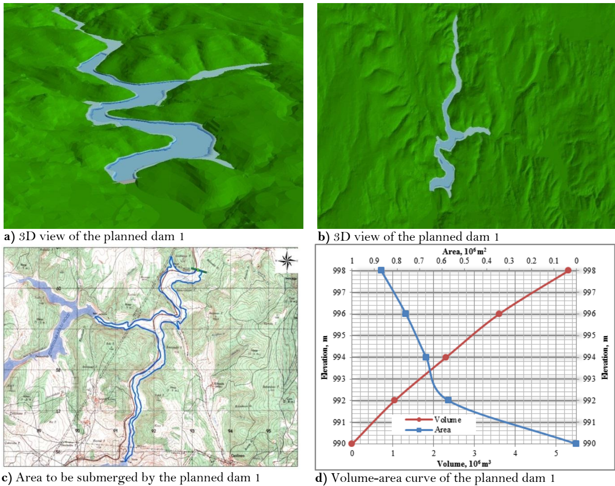
Figure-13. View and Area Features of the Planned Dam 1.
