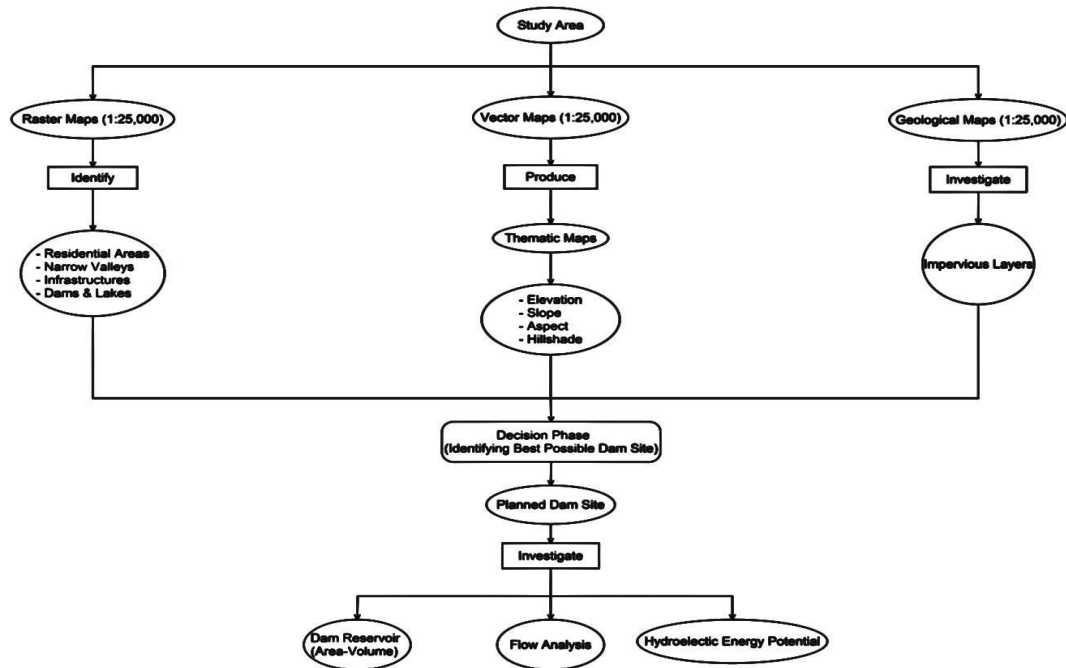
Figure-2. Flowchart of classical method.
