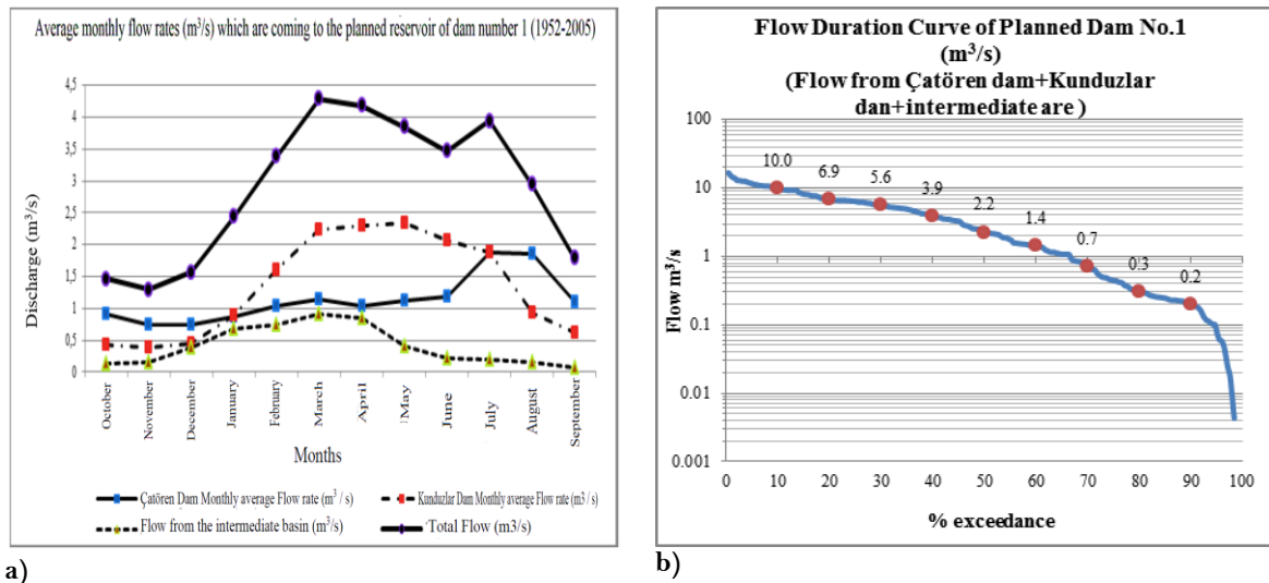
Figure-12. Flows of planned dam a) Inflow to Reservoir of the Planned Dam No.1 b)Flow duration Curve of the planned dam no.1.
