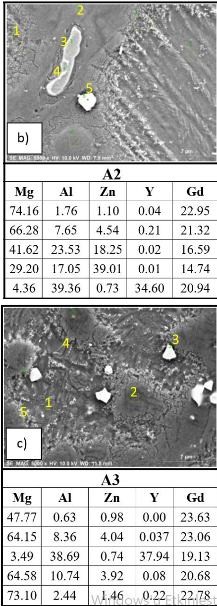
Şekil 5. (devamı). b) AZ31+ 0.5%Gd+0.5%Y, c) AZ31+1%Gd+1%Y, (A1-A3 SEM Images a) AZ31, b) AZ31+0.5%Gd+0.5%Y, c) AZ31+1%Gd+1%Y)
