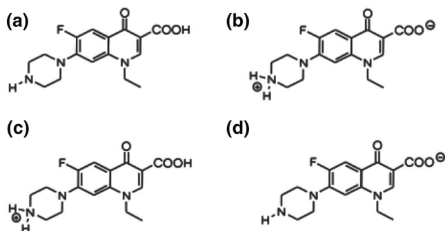
FIGURE 2 Different ionized and non-ionized forms of norfloxacin
