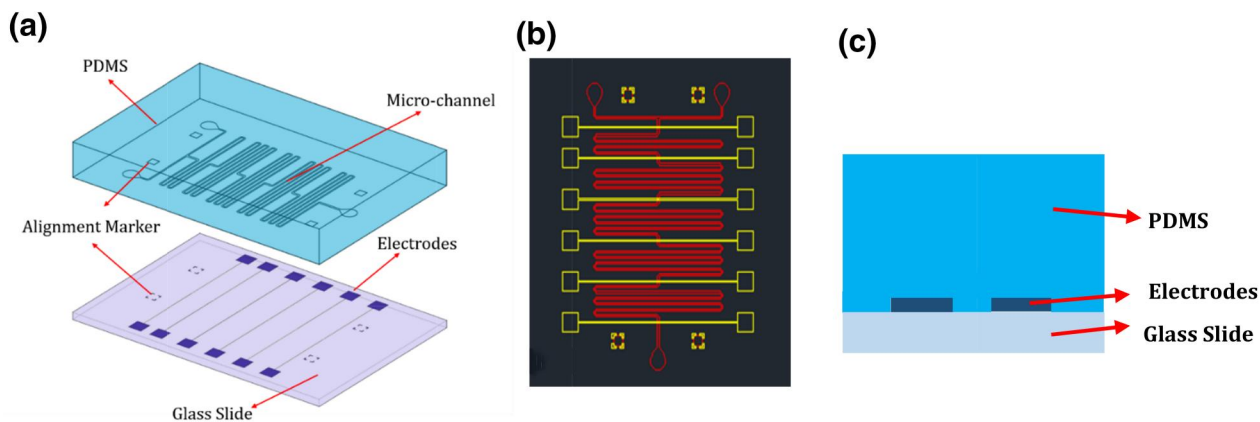
FIGURE 3 a) 3D view of the integrated chip. (b) 2D view represents the cross section of electrodes and microchannels. (c) Schematic of the cross section of the integrated chip
