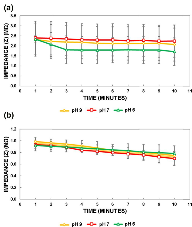
FIGURE 5 Impedance results for bilayer and porin-mediated permeation at different pH: (a) bilayer permeation; (b) porin-mediated permeation. Error bars represent standard error of the mean ( n = 4 ), p > 0.05
